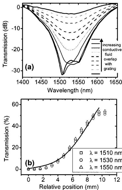
FIG. 3. (a) Evolution of the transmission spectrum as the conductive plug (water with ionic salt) advances over the LPG optimized for TAP in silicone oil. As the conductive fluid overlaps gradually over grating structure, the resonance feature disappears. (b) The variation of the transmitted intensity as a function of relative position of the conductive fluid over the grating structure for different wavelengths. The solid lines are the theoretical fits to the experimental data using Eq. (1) with \kappa=0.1538 , \delta_1=0 , and \delta_2=0.13791 .
