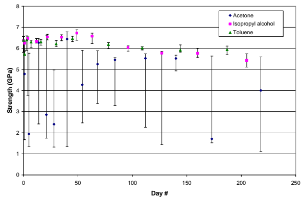
Figure 2: Acrylate fiber aging behavior in chemicals
