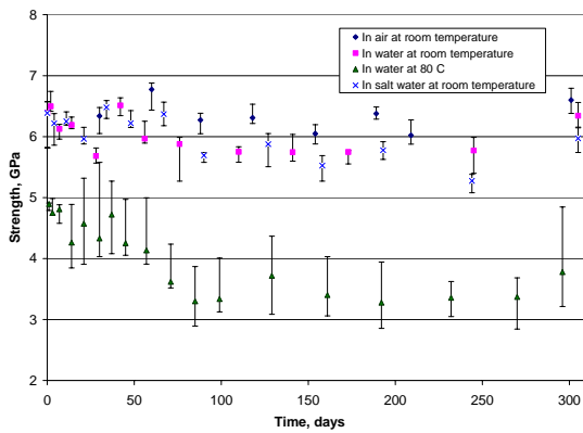
Figure 1: Acrylate fiber aging behavior in water
